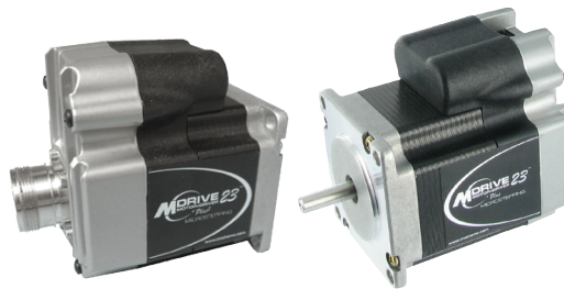
MDM•23 MDrive Plus Step/direction input products: integrated NEMA23 motor and controls, IP65 & IP20-rated
